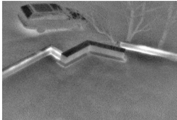
Figure 2: Convection heat loss from exterior wall/flat roof perimeter detail, due to lack of continuous wall/roof air barrier.
