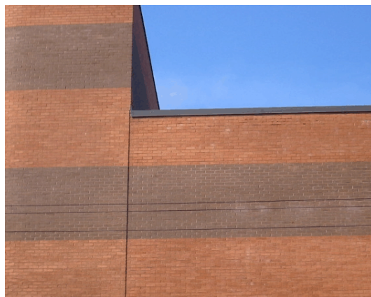
Figure 3: Convection heat loss at wall corner/flat roof perimeter detail. Masonry brick wall appears to be wet, due to moist warm air ex-filtrating through exterior wall system.
